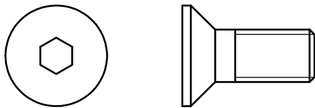
(A8)M10X25L SOCKER FLAT SCREW QTY.8
